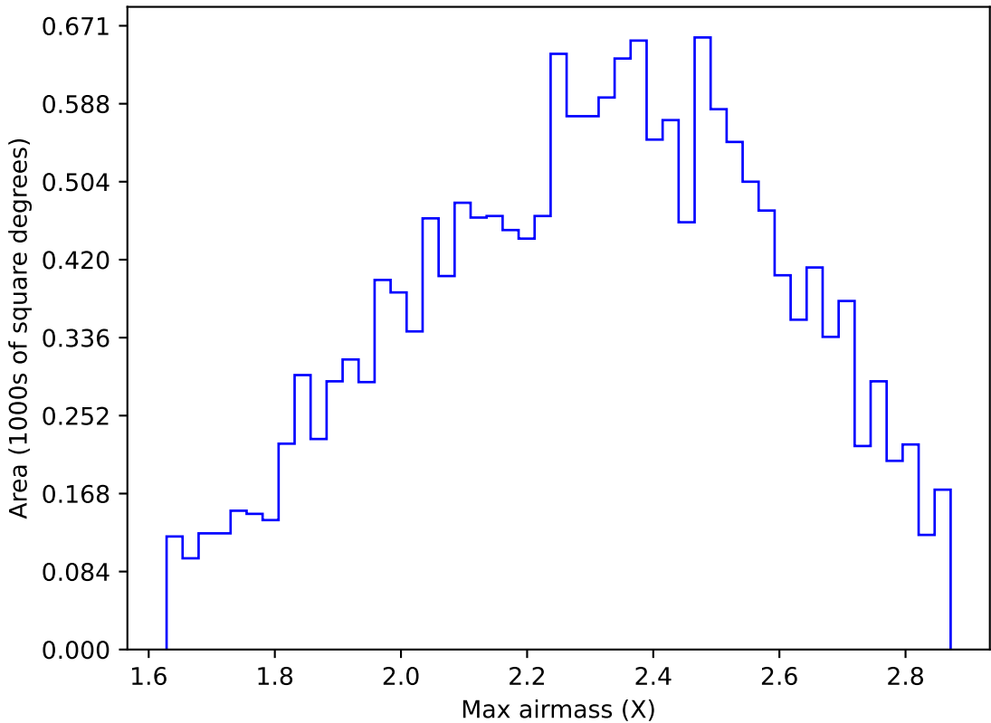
too_elab_2yr_r32_d2_ugrizy_v3.4_10yrs WFD y band: Max airmass
