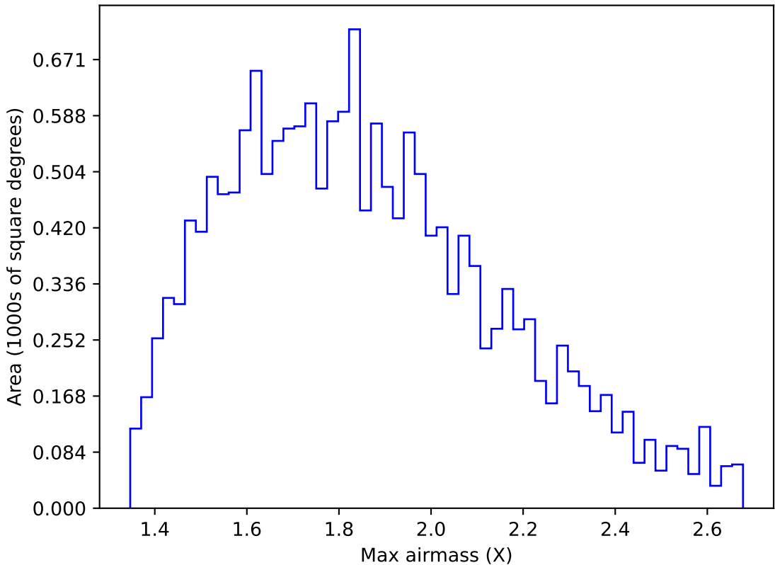
too_elab_2yr_r32_d2_ugrizy_v3.4_10yrs WFD u band: Max airmass
