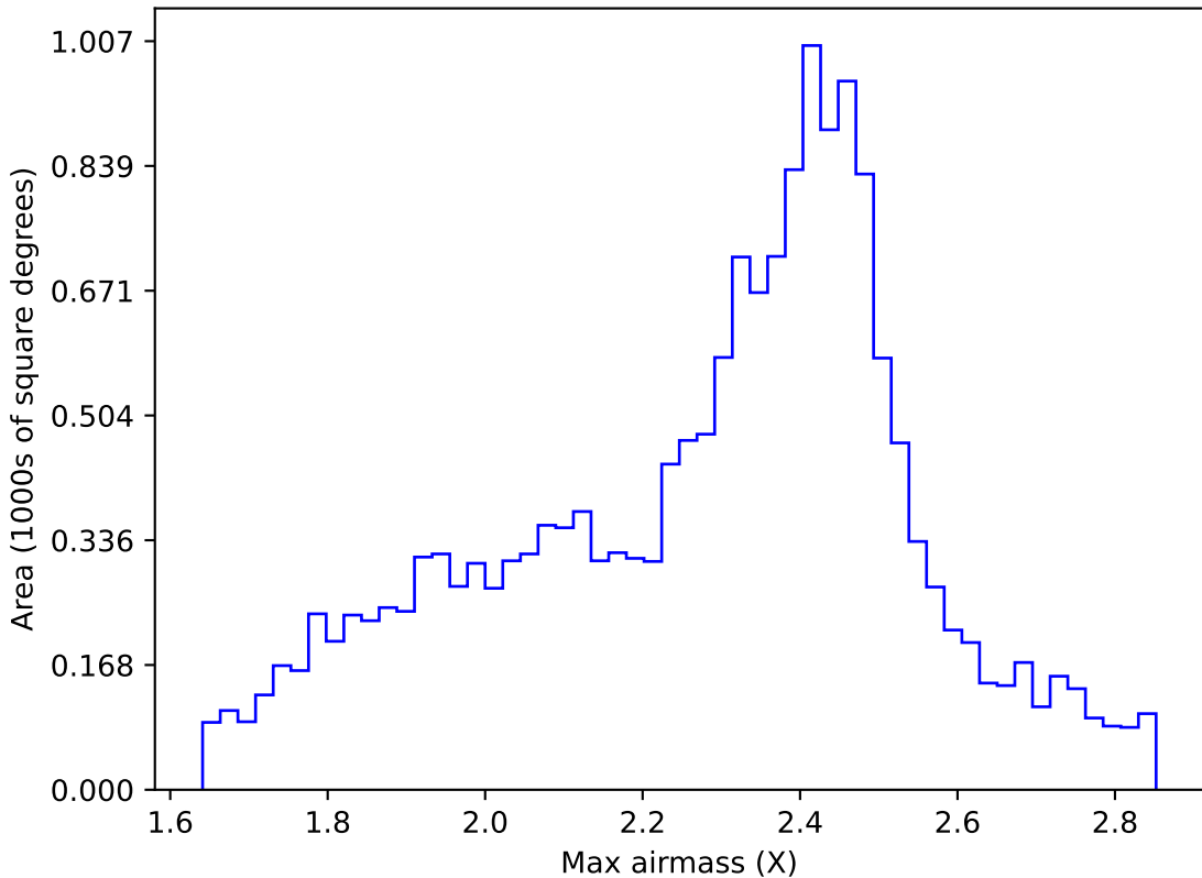
too_elab_2yr_r32_d2_ugrizy_v3.4_10yrs WFD r band: Max airmass
