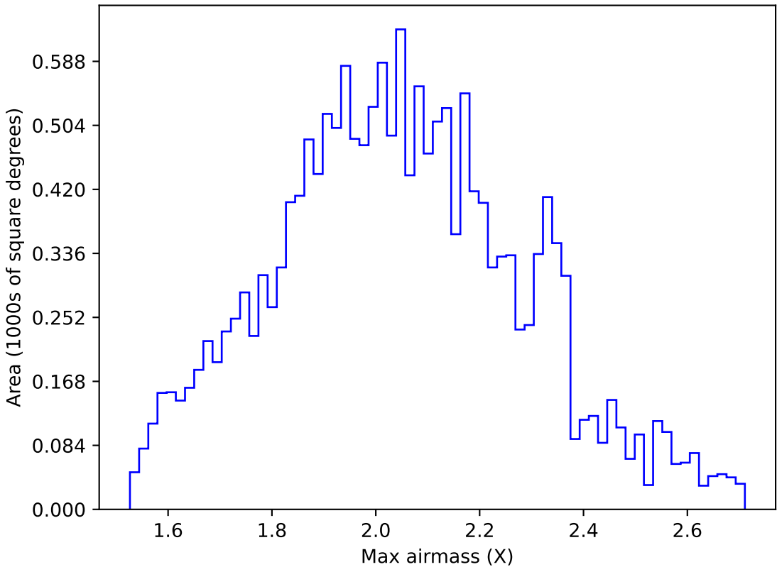
too_elab_2yr_r32_d2_ugrizy_v3.4_10yrs WFD g band: Max airmass
