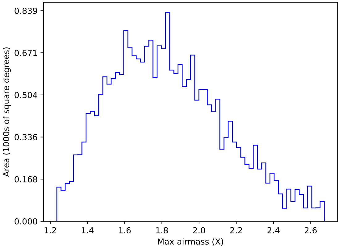
too_elab_2yr_r32_d2_ugrizy_v3.4_10yrs All sky u band: Max airmass
