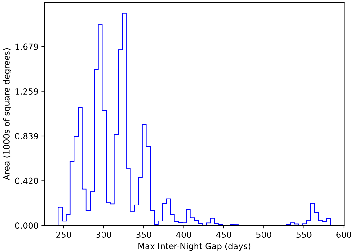
too_elab_2yr_r32_d2_ugrizy_v3.4_10yrs WFD y band: Max Inter-Night Gap
