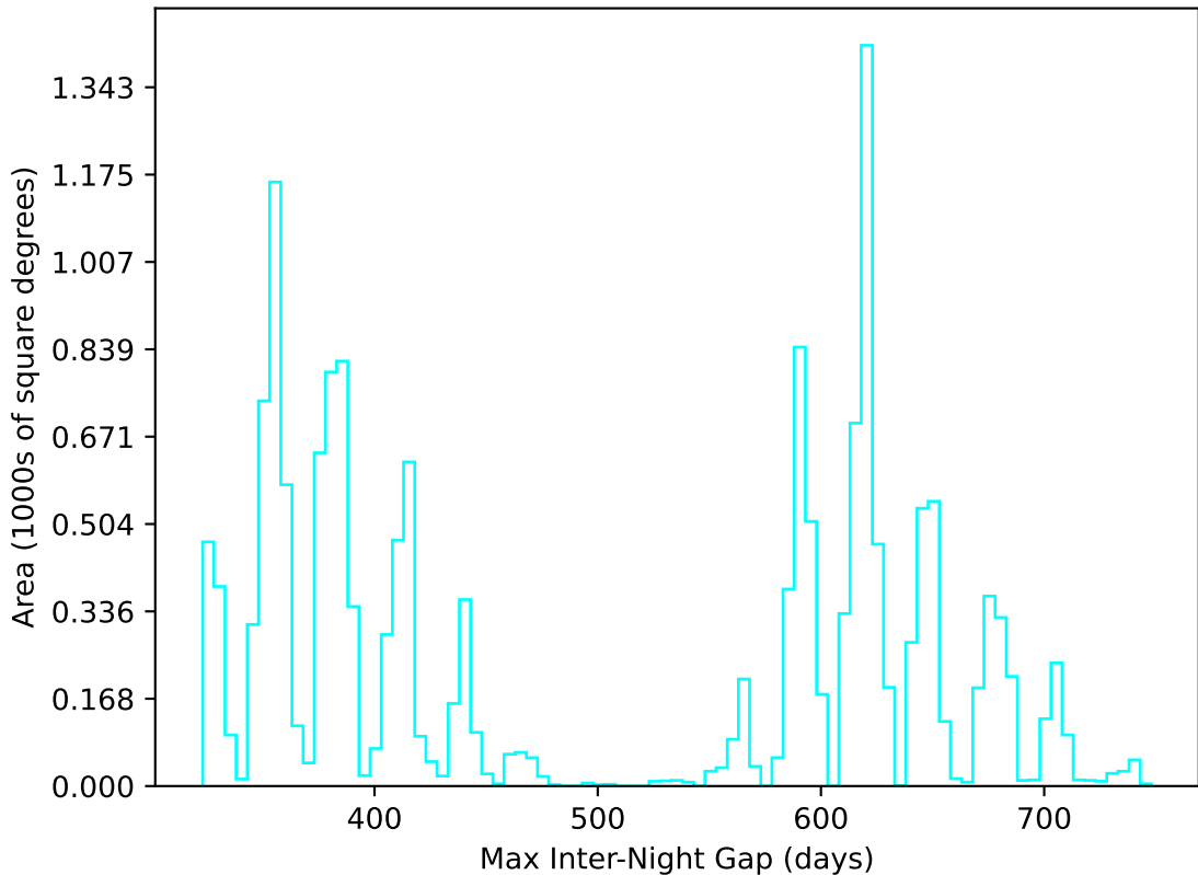
too_elab_2yr_r32_d2_ugrizy_v3.4_10yrs WFD u band: Max Inter-Night Gap
