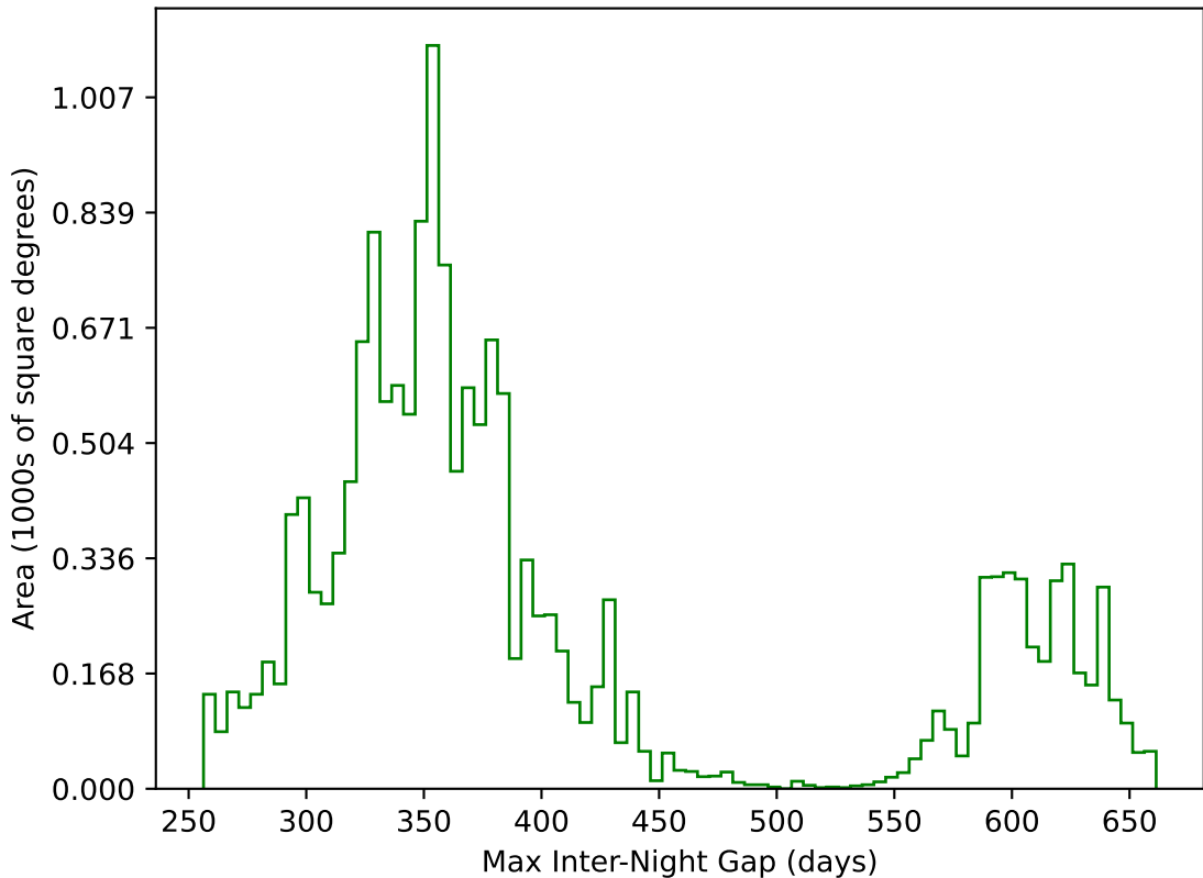
too_elab_2yr_r32_d2_ugrizy_v3.4_10yrs WFD g band: Max Inter-Night Gap
