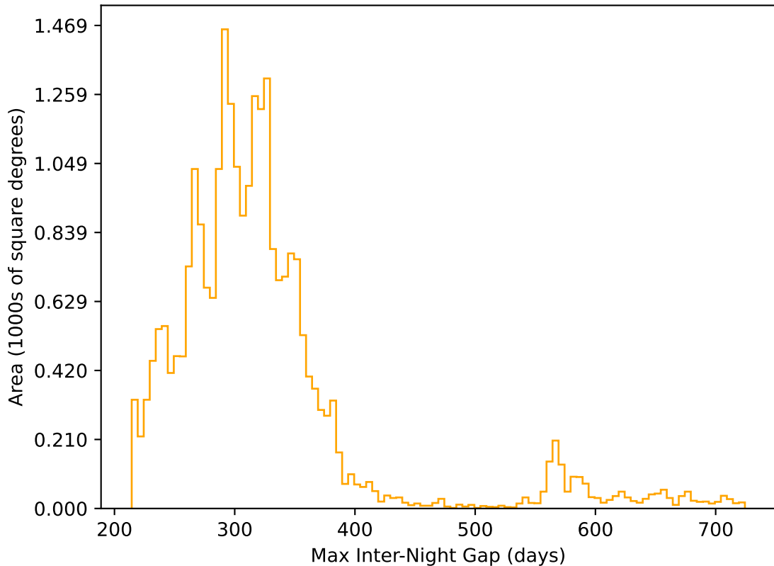
too_elab_2yr_r32_d2_ugrizy_v3.4_10yrs All sky r band: Max Inter-Night Gap
