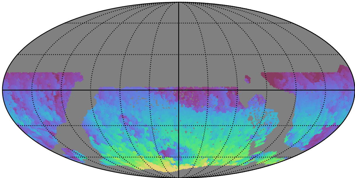
too_elab_2yr_r32_d2_ugrizy_v3.4_10yrs WFD z band: Max HA
