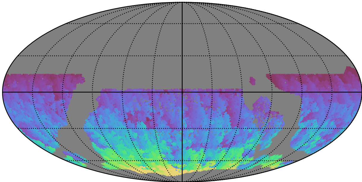
too_elab_2yr_r32_d2_ugrizy_v3.4_10yrs WFD y band: Max HA
