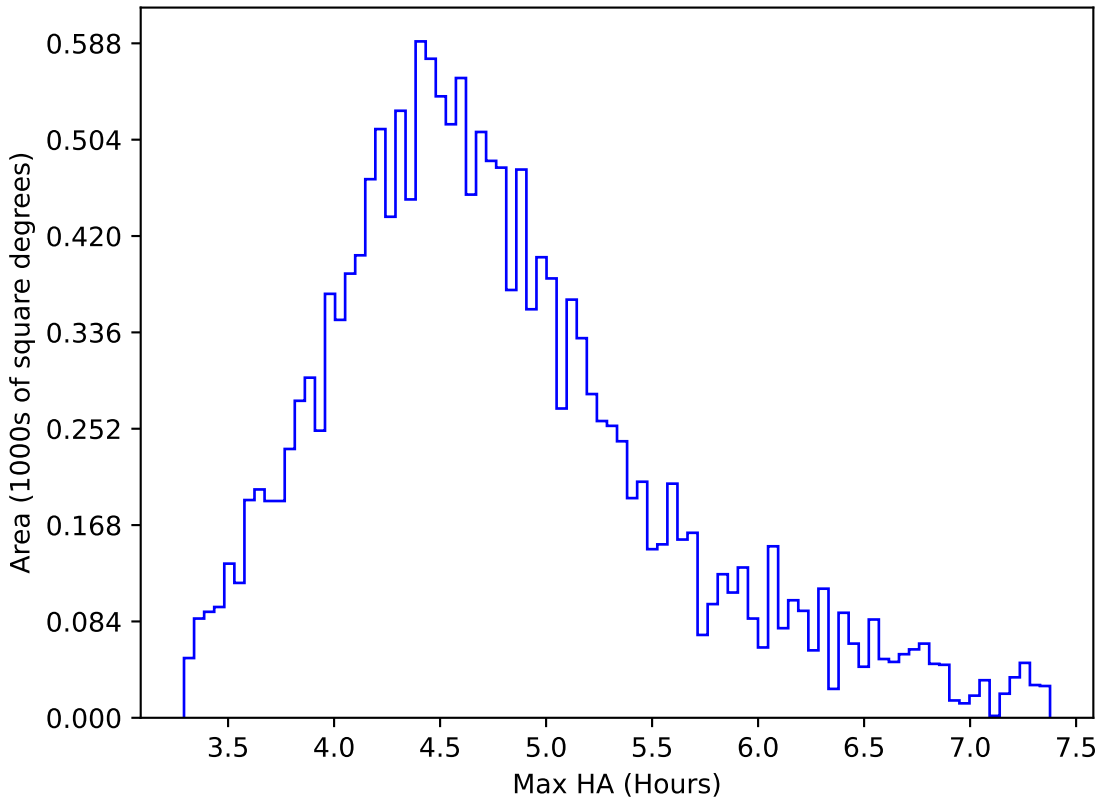
too_elab_2yr_r32_d2_ugrizy_v3.4_10yrs WFD y band: Max HA
