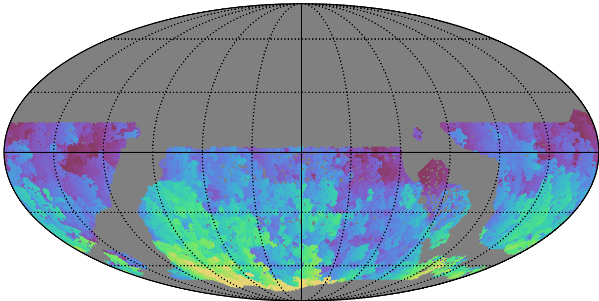
too_elab_2yr_r32_d2_ugrizy_v3.4_10yrs WFD u band: Max HA
