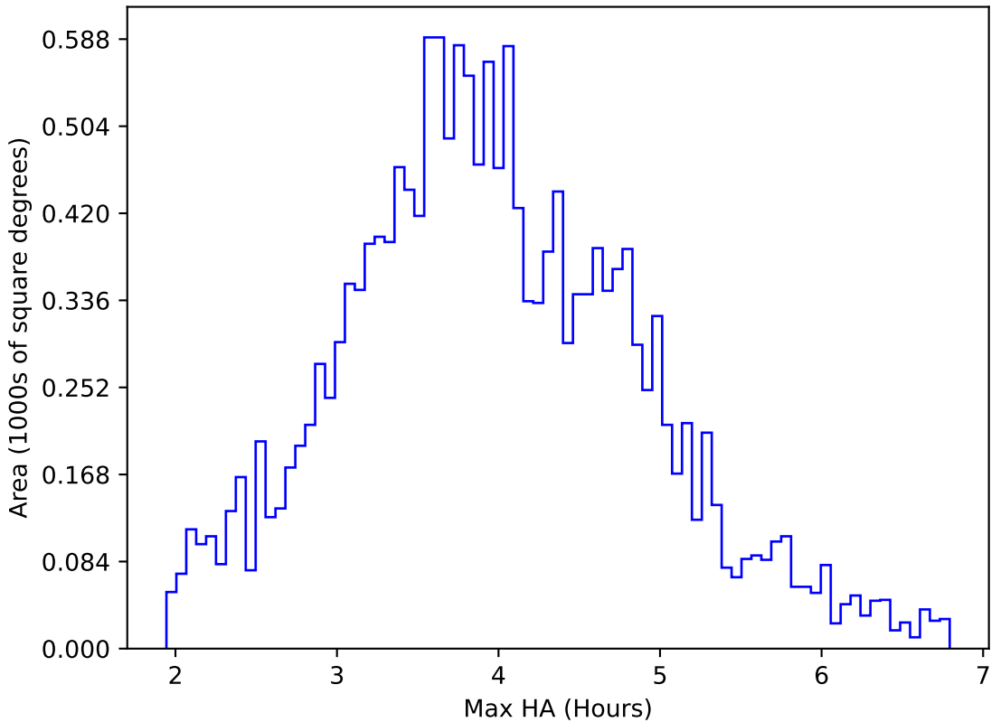
too_elab_2yr_r32_d2_ugrizy_v3.4_10yrs WFD u band: Max HA
