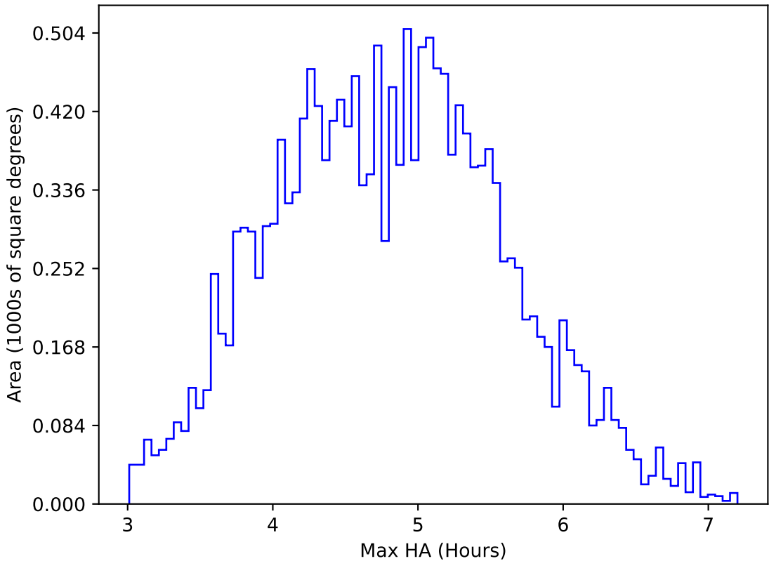
too_elab_2yr_r32_d2_ugrizy_v3.4_10yrs WFD i band: Max HA
