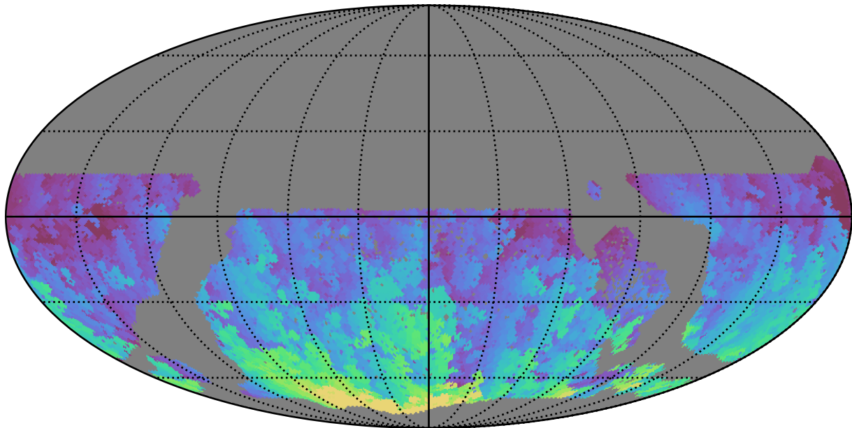
too_elab_2yr_r32_d2_ugrizy_v3.4_10yrs WFD g band: Max HA
