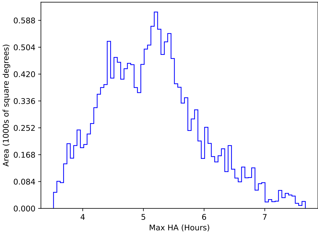
too_elab_2yr_r32_d2_ugrizy_v3.4_10yrs WFD all bands: Max HA
