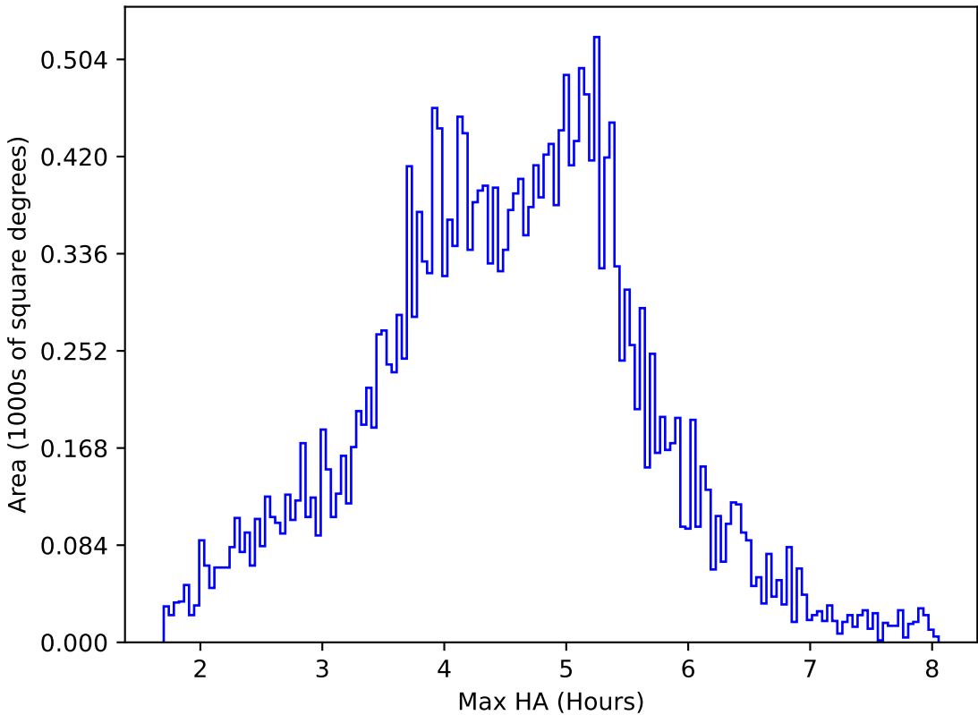
too_elab_2yr_r32_d2_ugrizy_v3.4_10yrs All sky z band: Max HA
