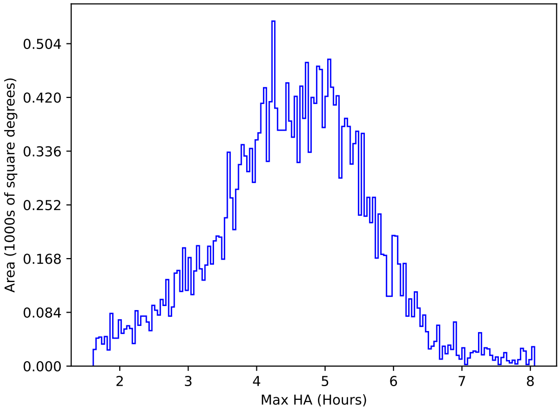
too_elab_2yr_r32_d2_ugrizy_v3.4_10yrs All sky i band: Max HA
