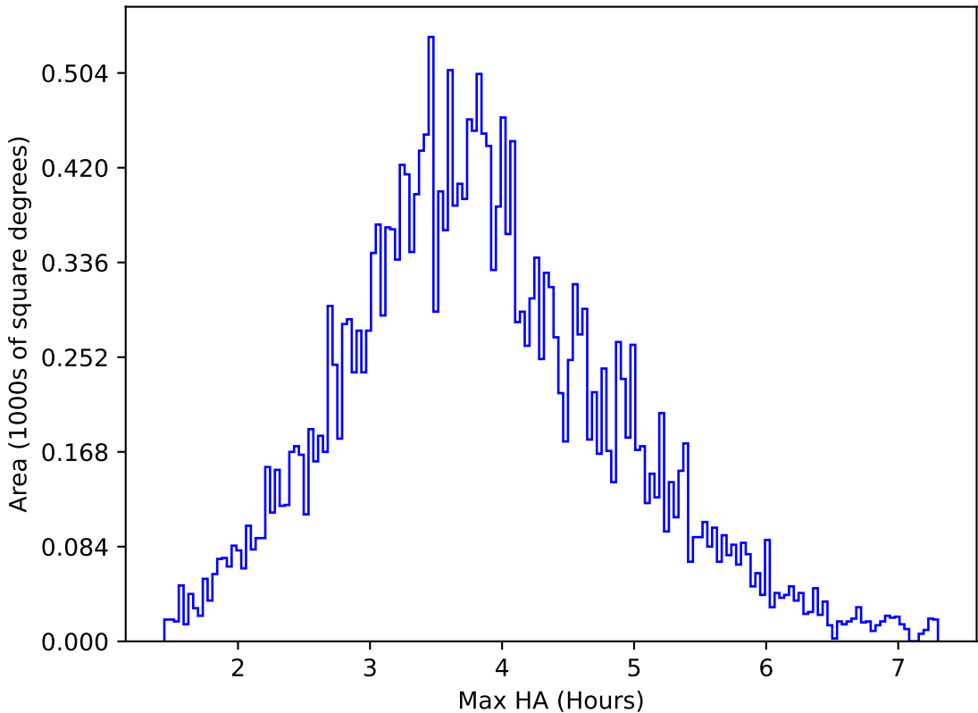
too_elab_2yr_r32_d2_ugrizy_v3.4_10yrs All sky g band: Max HA
