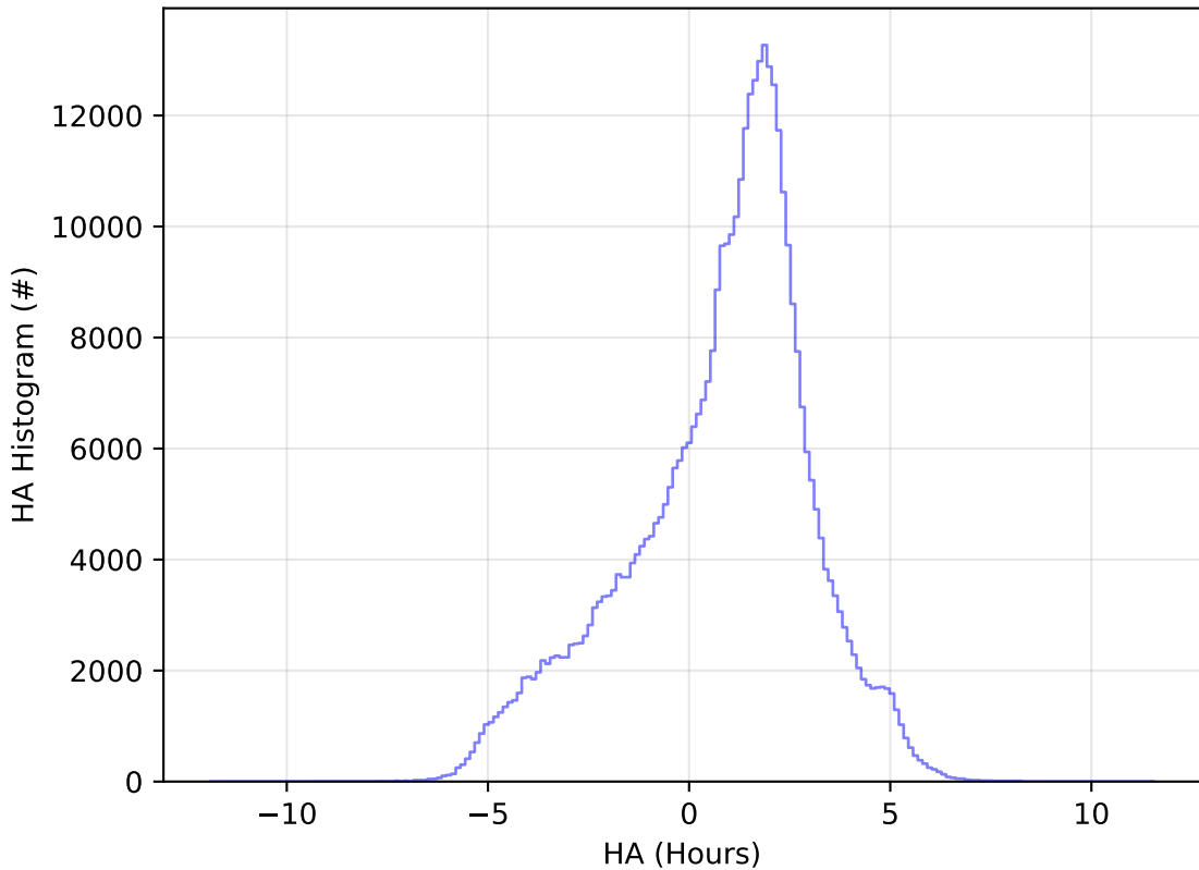
too_elab_2yr_r32_d2_ugrizy_v3.4_10yrs WFD z band: HA Histogram
