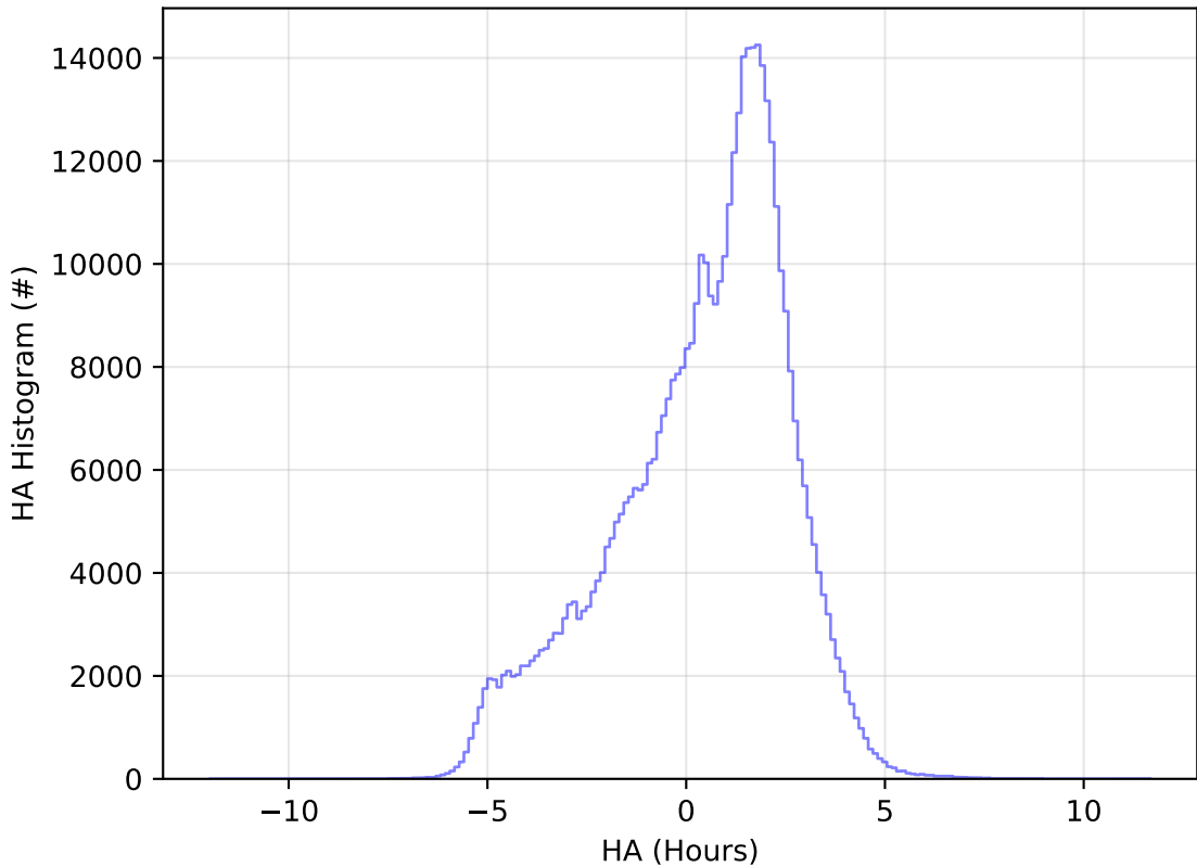
too_elab_2yr_r32_d2_ugrizy_v3.4_10yrs WFD r band: HA Histogram
