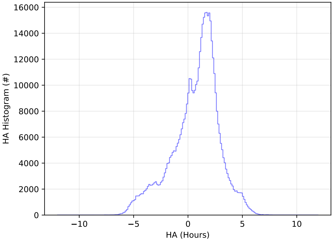
too_elab_2yr_r32_d2_ugrizy_v3.4_10yrs WFD i band: HA Histogram
