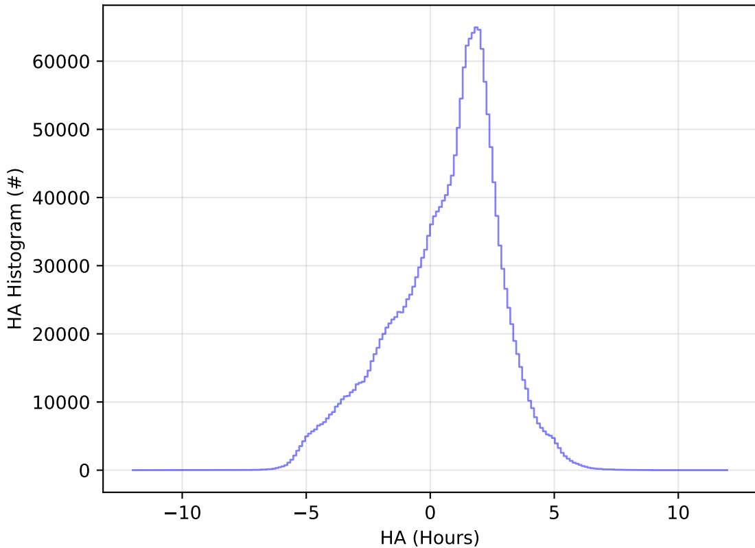
too_elab_2yr_r32_d2_ugrizy_v3.4_10yrs WFD all bands: HA Histogram
