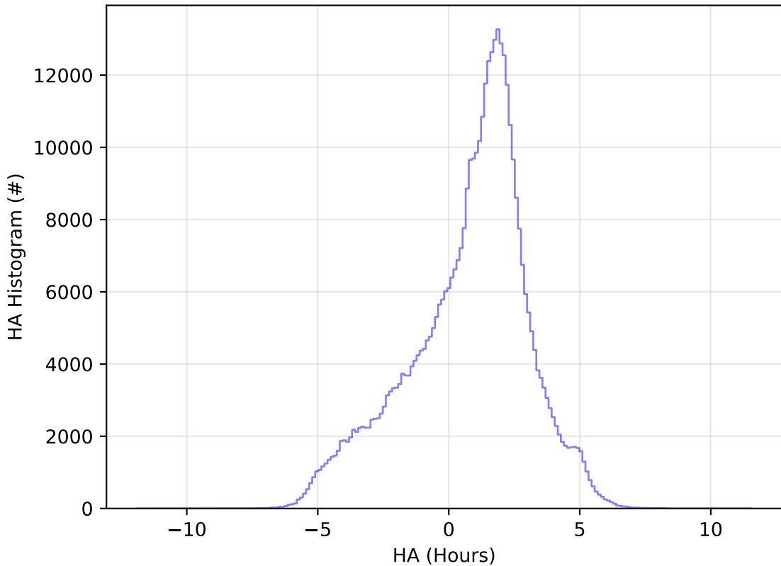
too_elab_2yr_r32_d2_ugrizy_v3.4_10yrs All sky z band: HA Histogram
