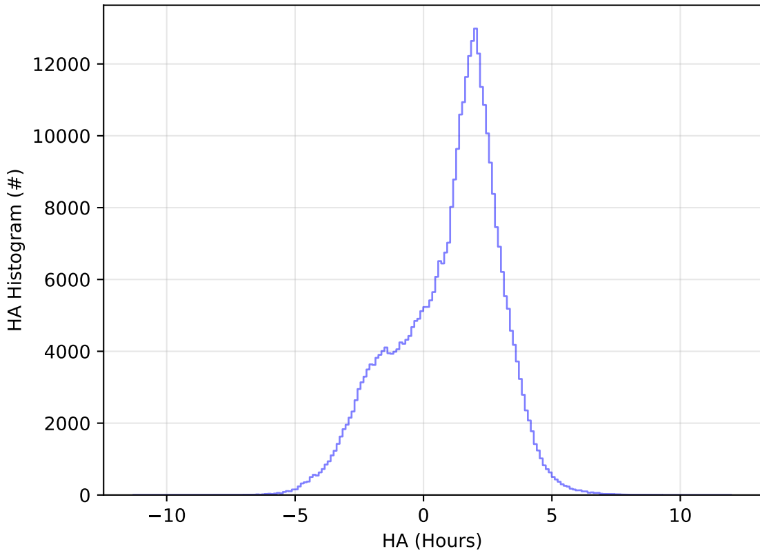
too_elab_2yr_r32_d2_ugrizy_v3.4_10yrs All sky y band: HA Histogram
