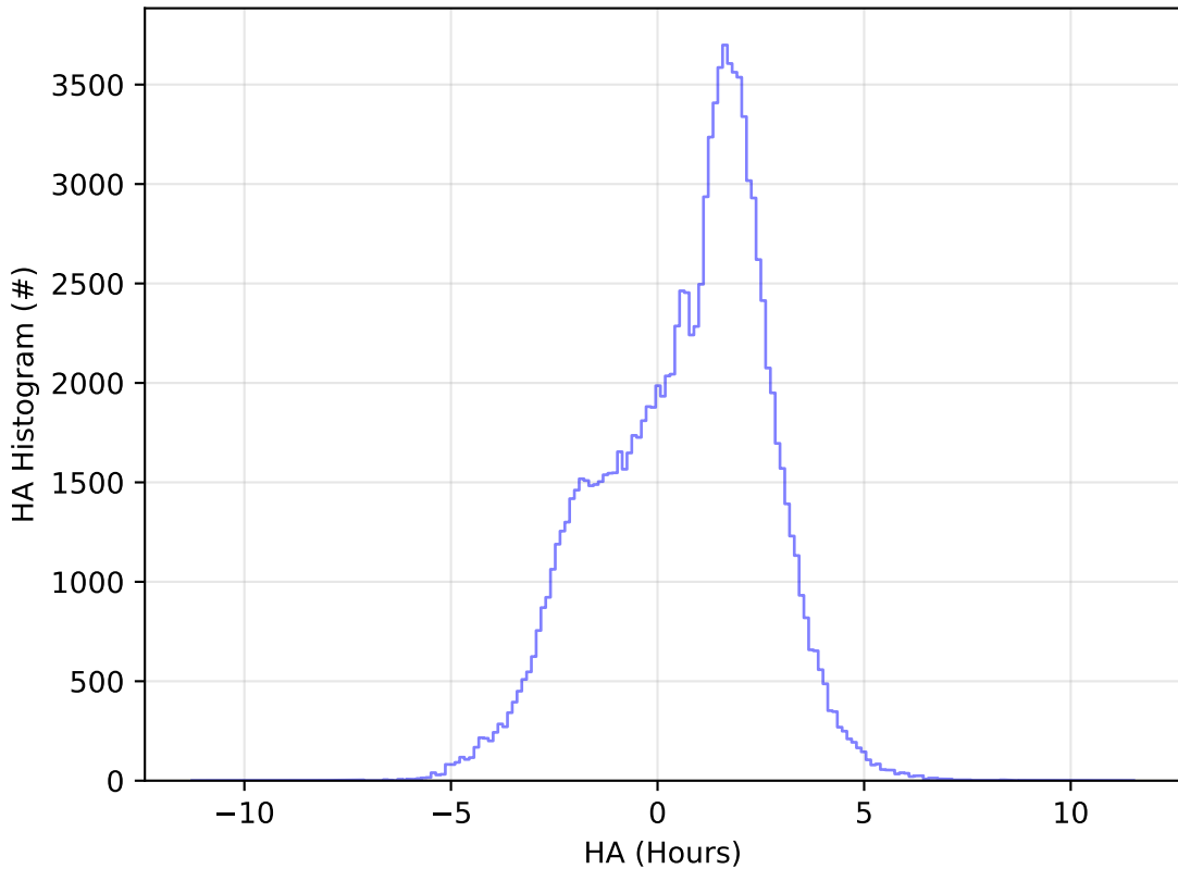
too_elab_2yr_r32_d2_ugrizy_v3.4_10yrs All sky u band: HA Histogram
