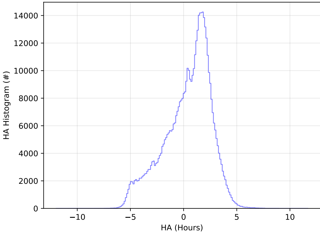
too_elab_2yr_r32_d2_ugrizy_v3.4_10yrs All sky r band: HA Histogram
