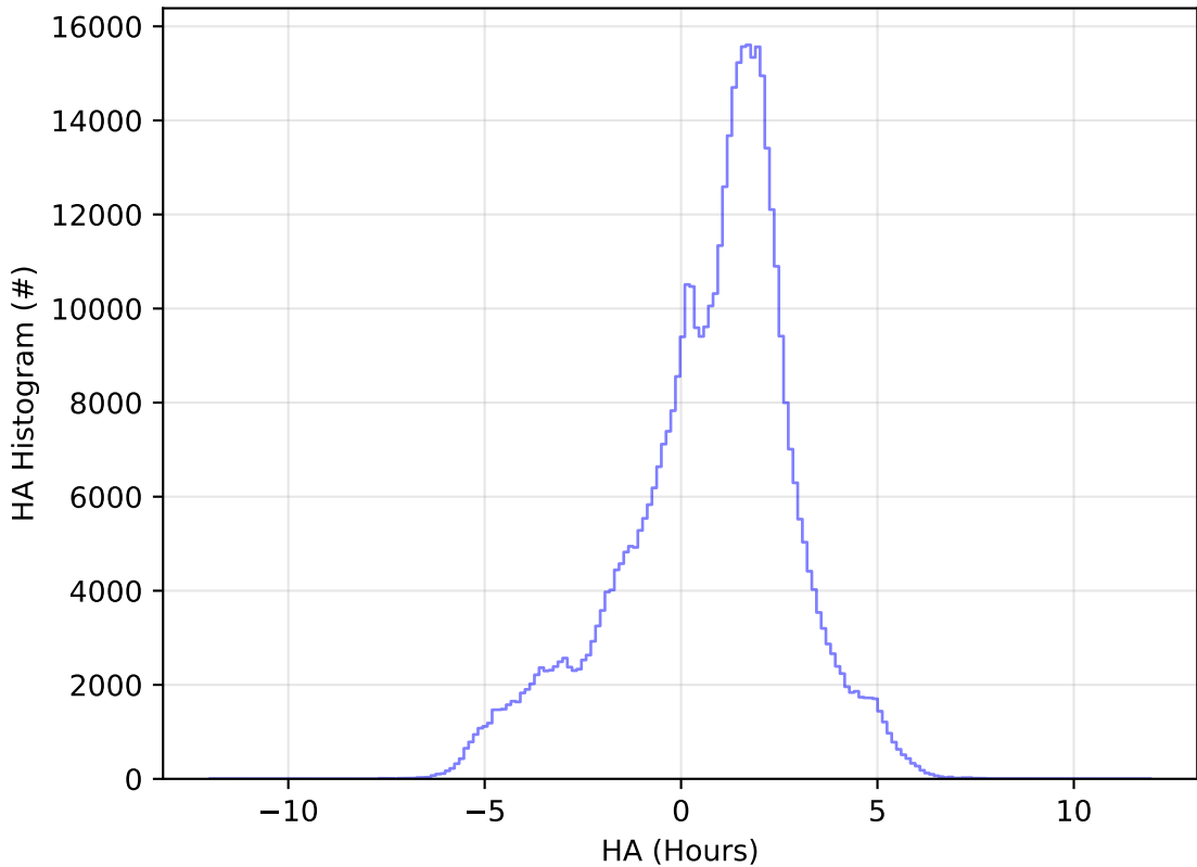
too_elab_2yr_r32_d2_ugrizy_v3.4_10yrs All sky i band: HA Histogram
