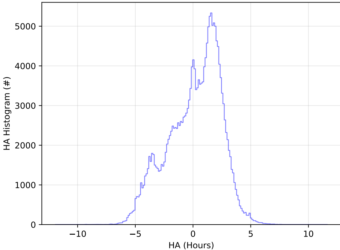
too_elab_2yr_r32_d2_ugrizy_v3.4_10yrs All sky g band: HA Histogram
