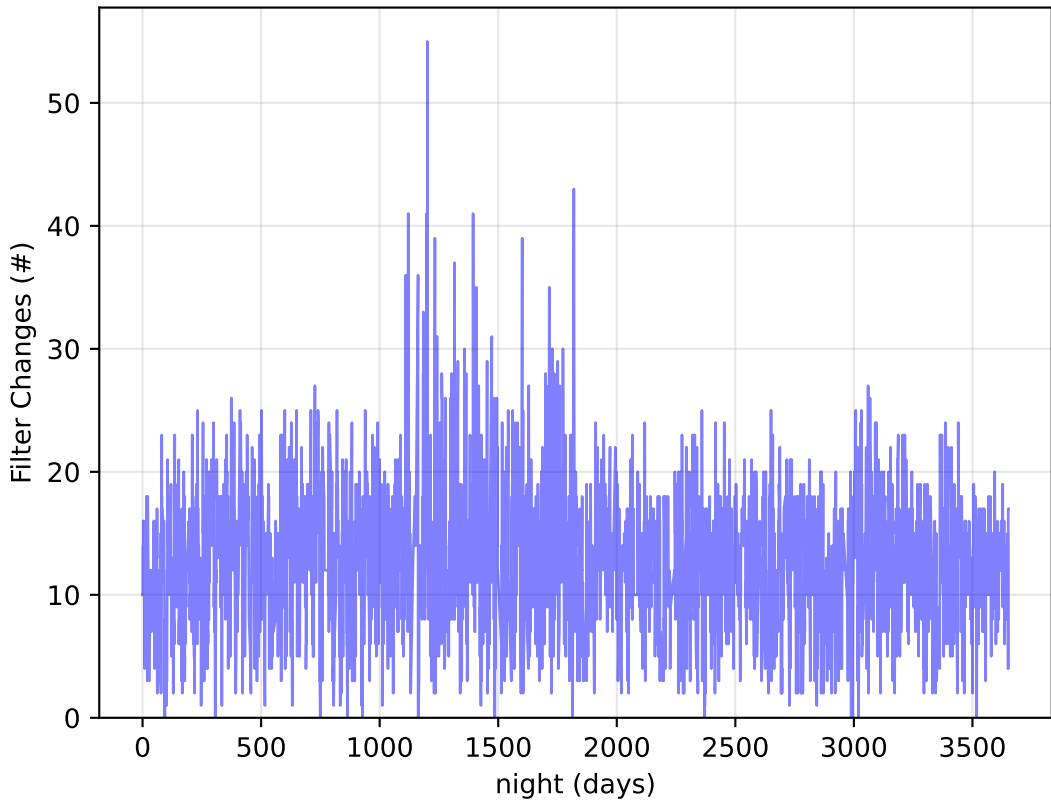
too_elab_2yr_r32_d2_ugrizy_v3.4_10yrs Per Night: Filter Changes
