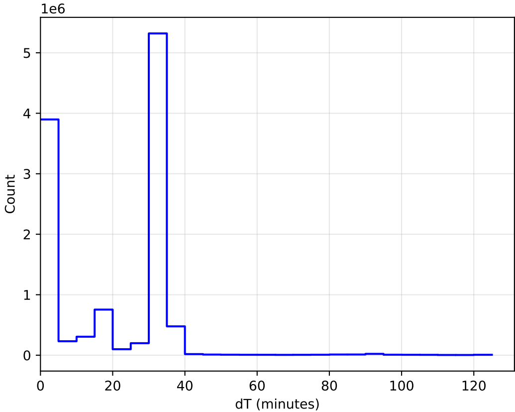
too_elab_2yr_r32_d2_ugrizy_v3.4_10yrs WFD: DeltaT Histogram
