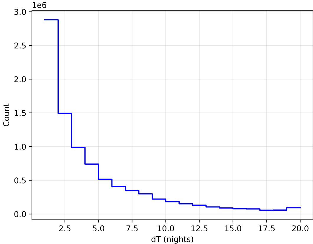
too_elab_2yr_r32_d2_ugrizy_v3.4_10yrs All sky all bands: DeltaNight Histogram
