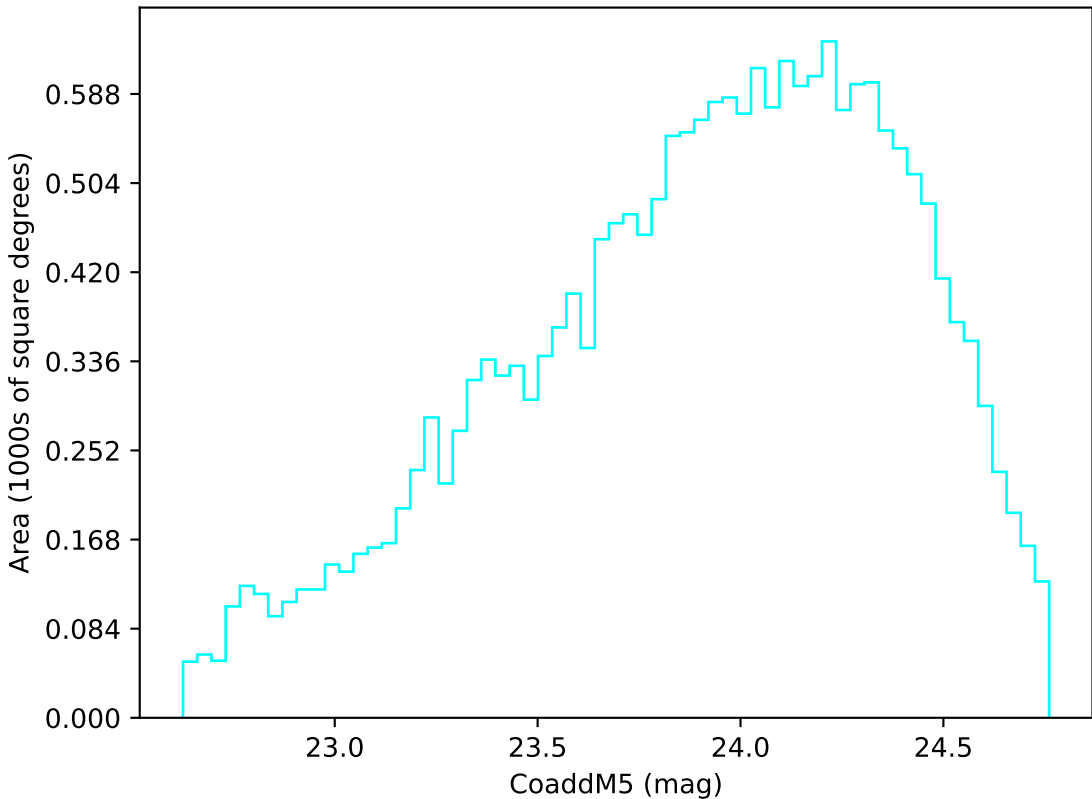
too_elab_2yr_r32_d2_ugrizy_v3.4_10yrs Yr 3-4 u band: CoaddM5
