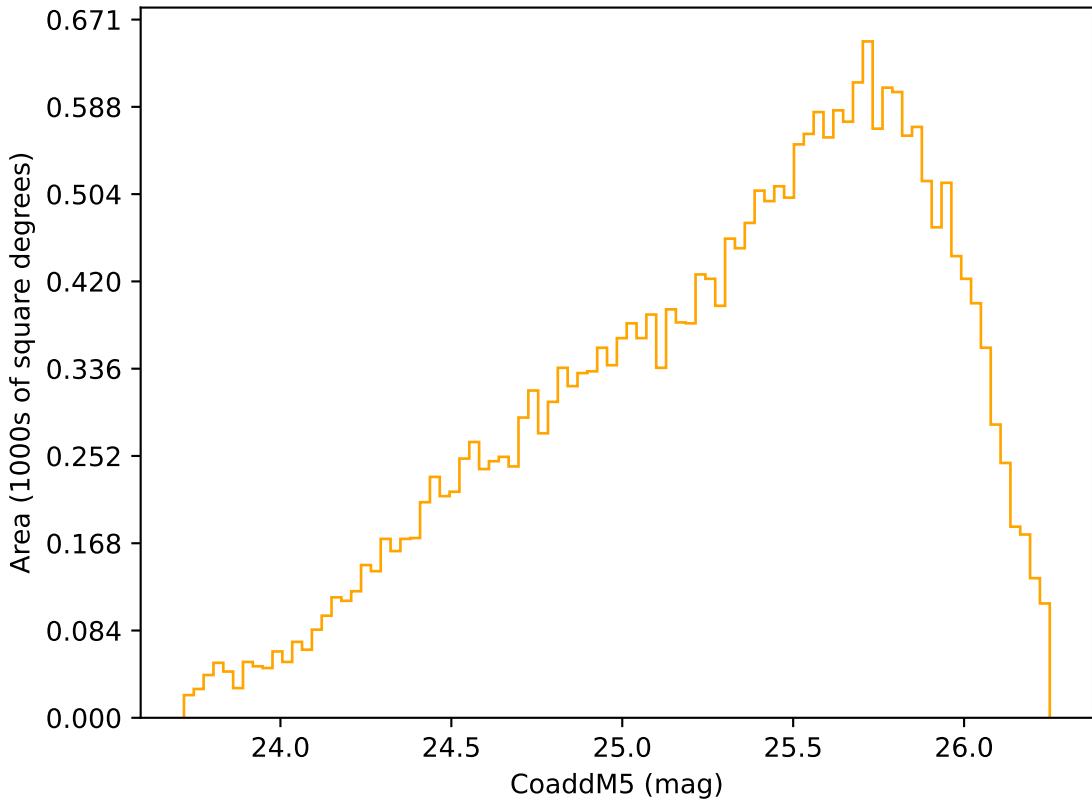
too_elab_2yr_r32_d2_ugrizy_v3.4_10yrs Yr 3-4 r band: CoaddM5
