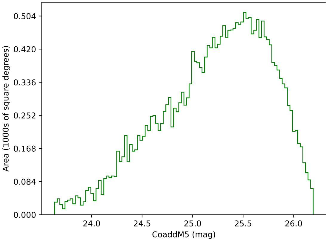
too_elab_2yr_r32_d2_ugrizy_v3.4_10yrs Yr 3-4 g band: CoaddM5
