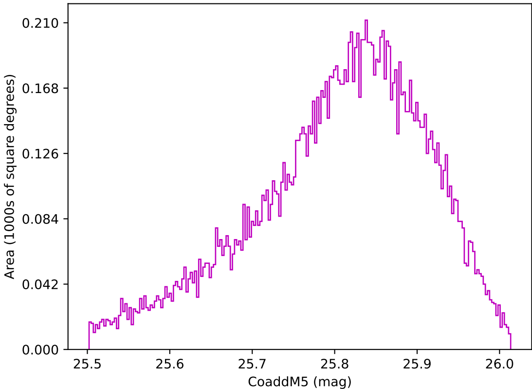
too_elab_2yr_r32_d2_ugrizy_v3.4_10yrs WFD z band: CoaddM5
