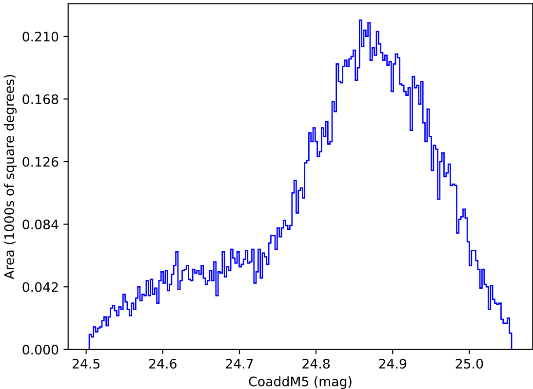
too_elab_2yr_r32_d2_ugrizy_v3.4_10yrs WFD y band: CoaddM5
