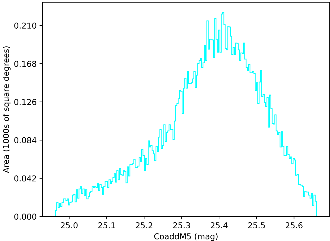
too_elab_2yr_r32_d2_ugrizy_v3.4_10yrs WFD u band: CoaddM5
