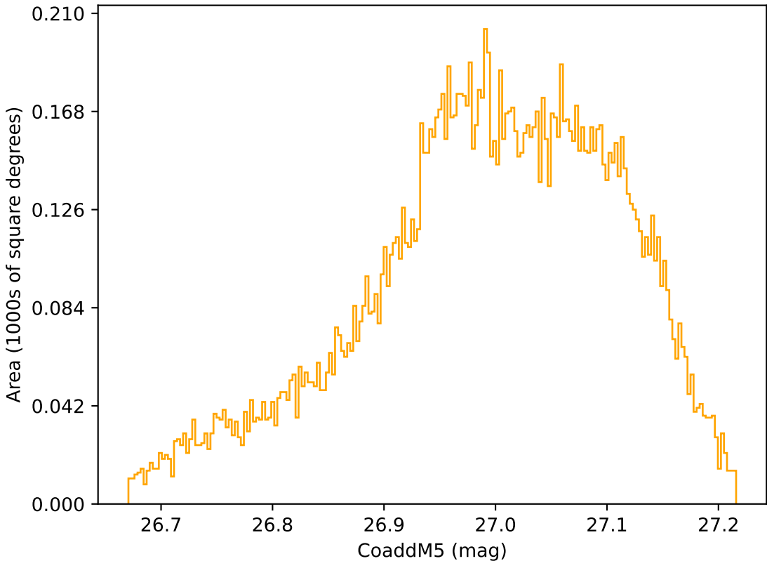
too_elab_2yr_r32_d2_ugrizy_v3.4_10yrs WFD r band: CoaddM5
