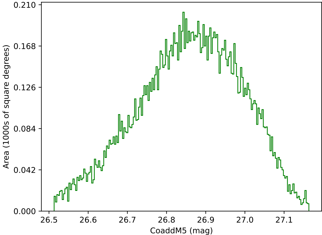
too_elab_2yr_r32_d2_ugrizy_v3.4_10yrs WFD g band: CoaddM5
