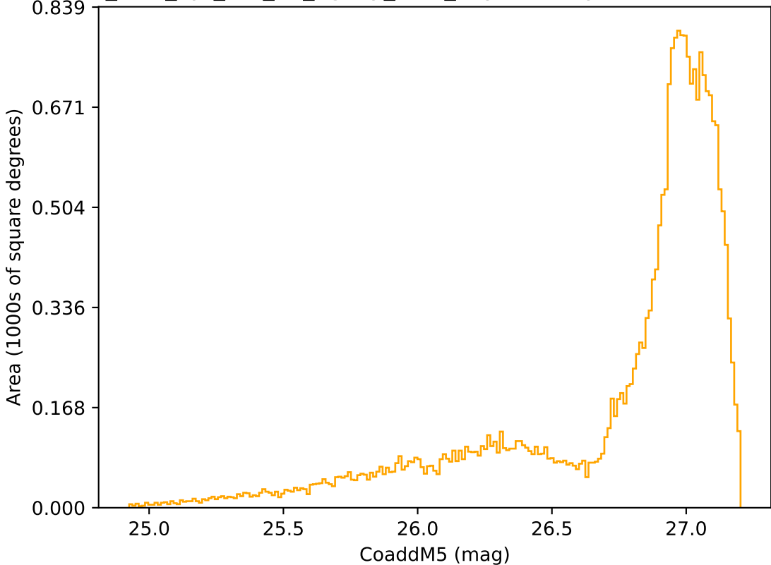
too_elab_2yr_r32_d2_ugrizy_v3.4_10yrs All sky r band: CoaddM5
