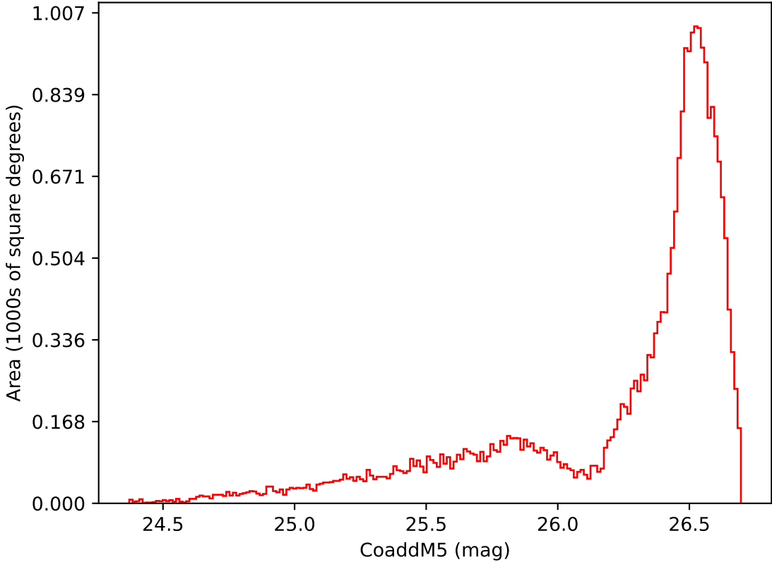
too_elab_2yr_r32_d2_ugrizy_v3.4_10yrs All sky i band: CoaddM5
