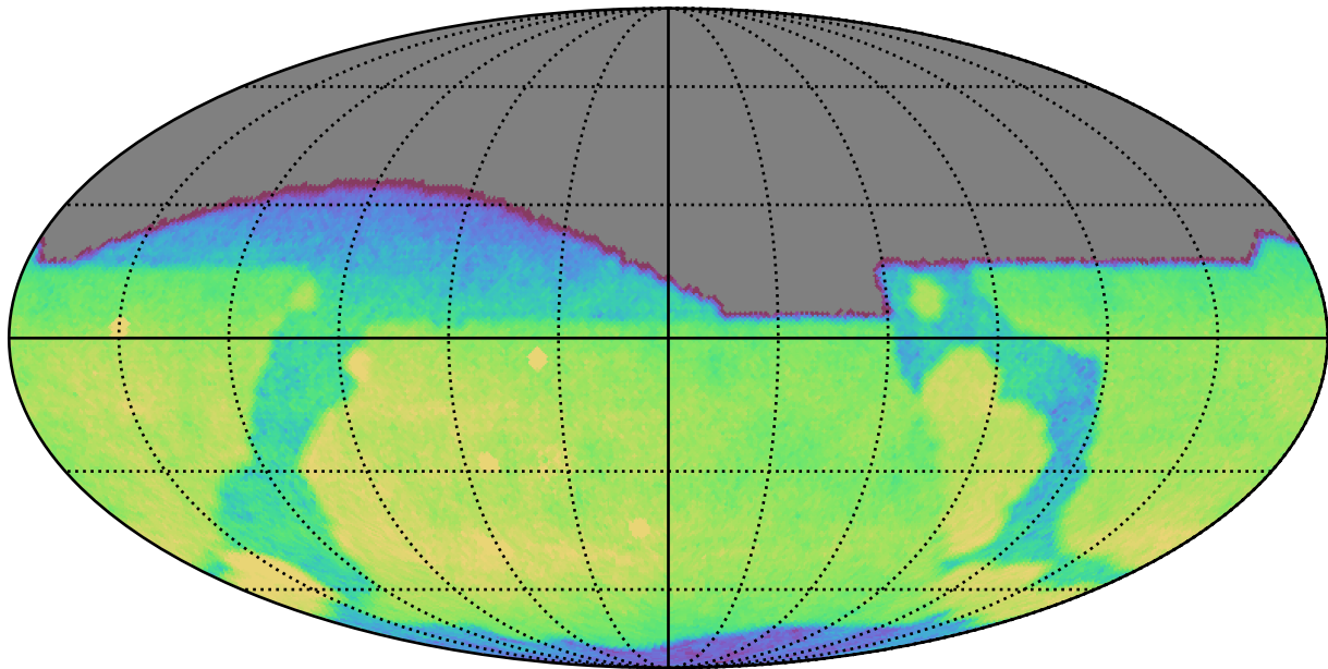
too_elab_2yr_r32_d2_ugrizy_v3.4_10yrs All sky g band: CoaddM5
