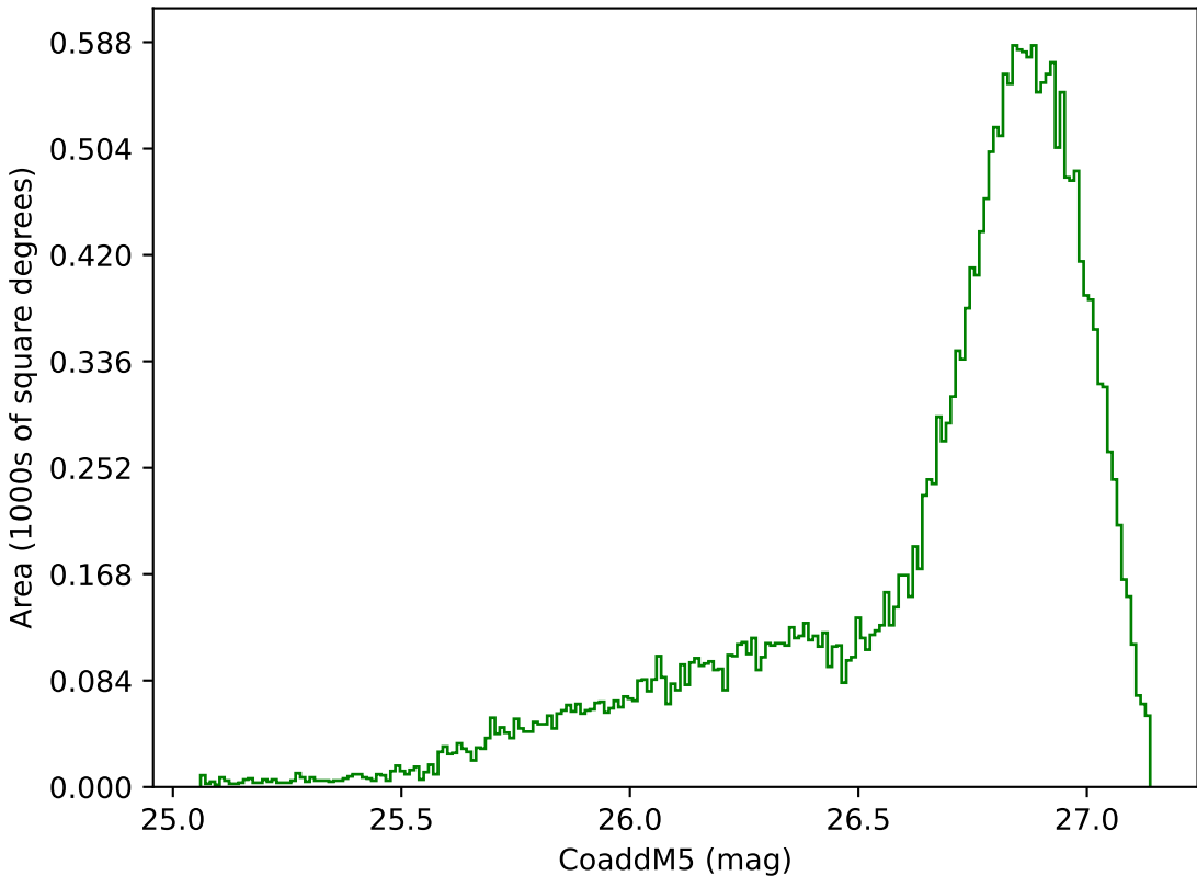
too_elab_2yr_r32_d2_ugrizy_v3.4_10yrs All sky g band: CoaddM5
