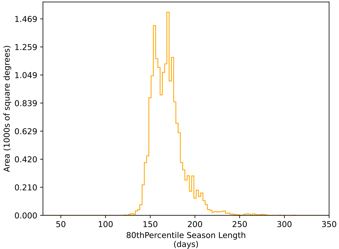
too_elab_2yr_r32_d2_ugrizy_v3.4_10yrs WFD r band: 80thPercentile Season Length
