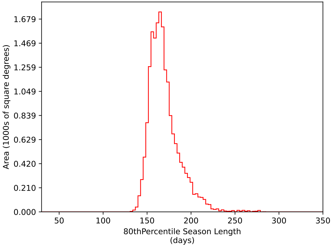
too_elab_2yr_r32_d2_ugrizy_v3.4_10yrs WFD i band: 80thPercentile Season Length
