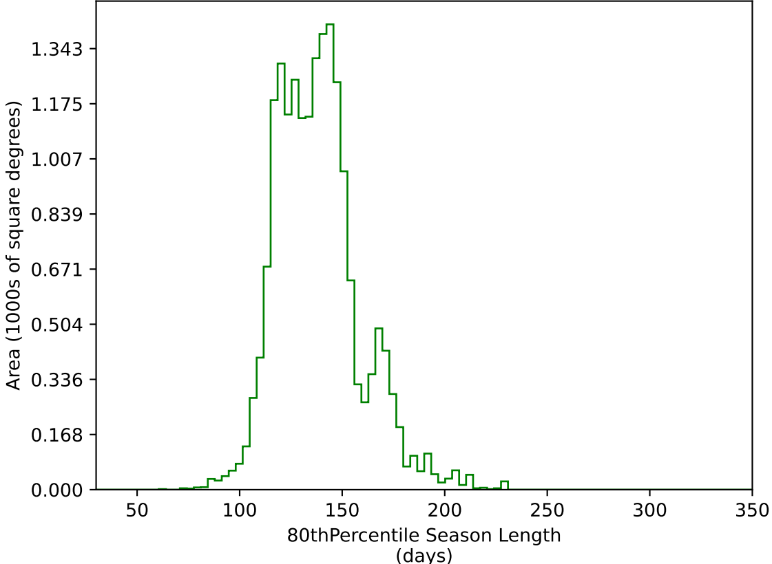
too_elab_2yr_r32_d2_ugrizy_v3.4_10yrs WFD g band: 80thPercentile Season Length
