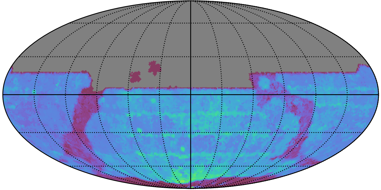
too_elab_2yr_r32_d2_ugrizy_v3.4_10yrs All sky y band: 80thPercentile Season Length
