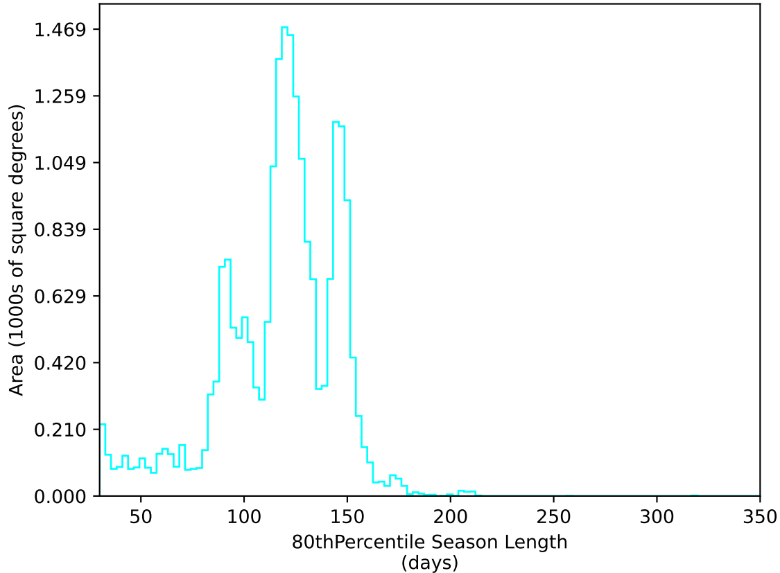
too_elab_2yr_r32_d2_ugrizy_v3.4_10yrs All sky u band: 80thPercentile Season Length
